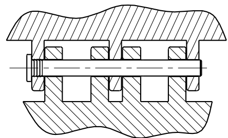
Application example: Latch Pin in Automotive Door Handle
